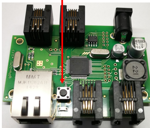
Reset gomb
